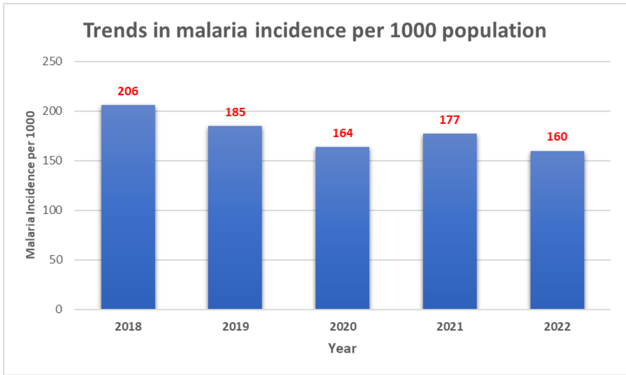
Figure 2: Malaria Incidence
