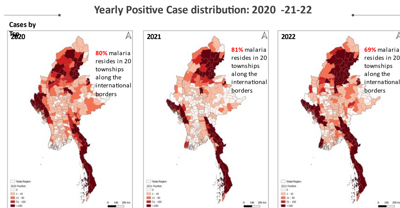
Figure 1: Incidence Maps
